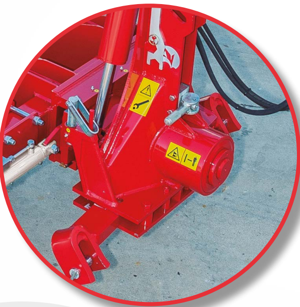
Oscillating cross shaft
